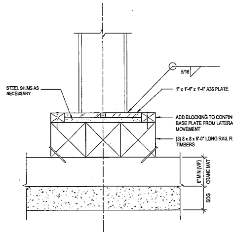
B1 DETAIL AT BASE
