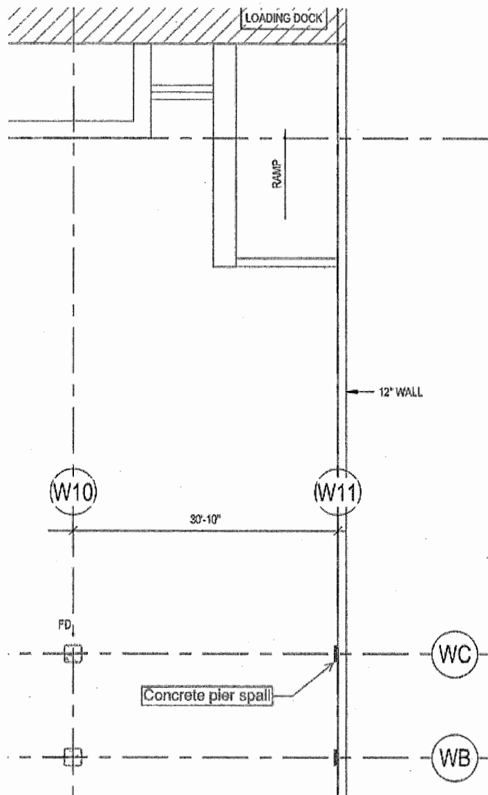
Figure 1. Spalled CIP concrete pier locations at West parking
