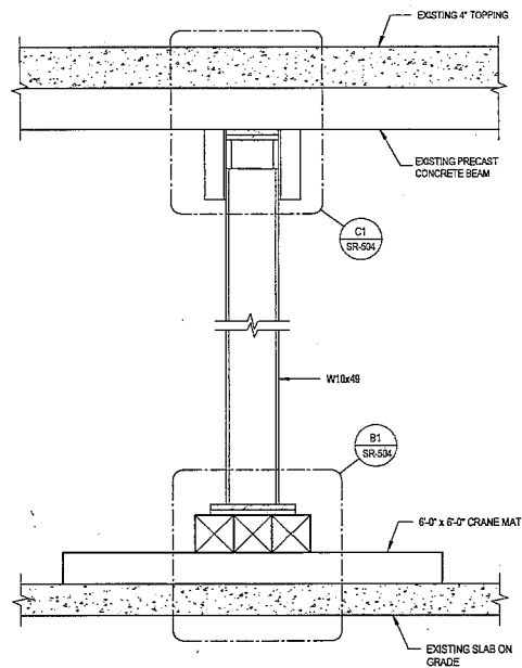
A1 SHORING ELEVATION
