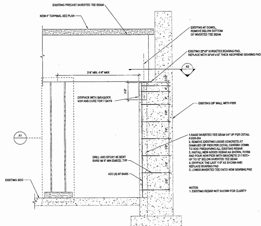
A2 ELEVATION VIEW OF CIP PIER REPAIR
