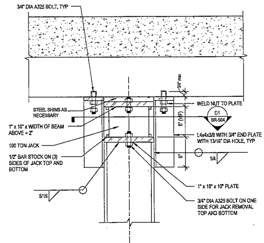
C1 DETAIL AT TOP
