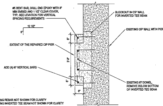
A3 TOP VIEW OF CIP PIER REPAIR
